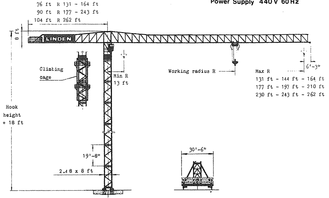
Rail mounted crane
